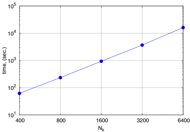
Fig. 2. A benchmark of \Theta\Phi , showing the dependence of the time for single self-consistency solution on the number of k -points along each of the dimensions of a 2D grid in the Brillouin zone. Note the logarithmic scale on both axes. Here, N_k is the number of k -points along each of the dimensions of a 2D grid in the Brillouin zone, so that in each grid there are N_k \times N_k points. U = 10t , T = 0.01t , ISS phase at Q = 0 .
