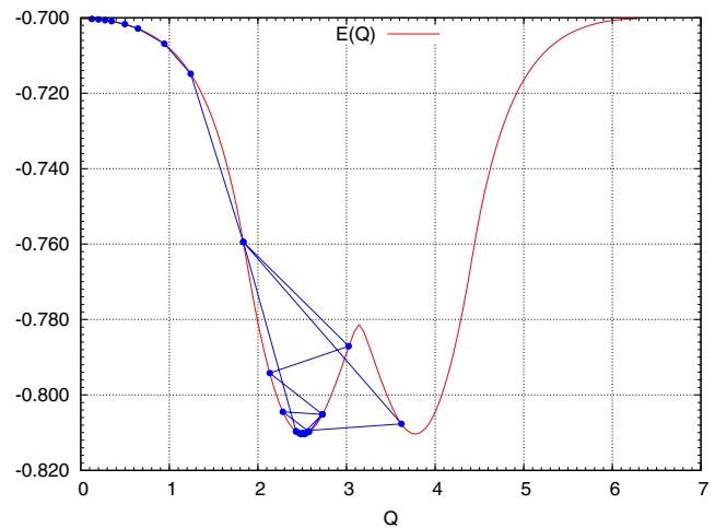
Fig. 1. A typical internal energy profile E(\mathbf{Q}) U = 5t , \delta = 0.15 , T = 0.0001t . E(\mathbf{Q}) has two local minima symmetric with respect to (\pi, \pi) , which is a local maximum. The blue line shows the simplex optimization within \Theta\Phi .
