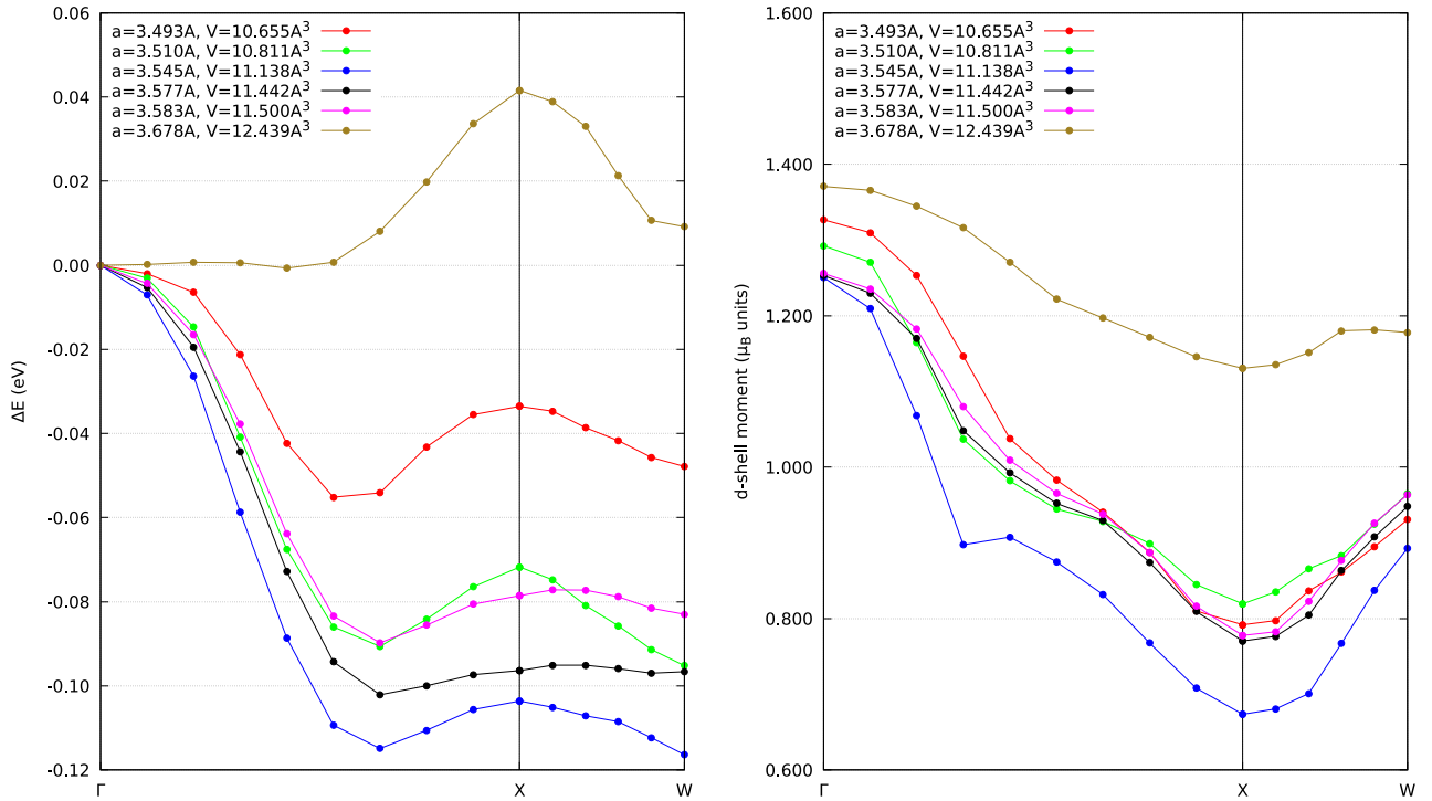
Fig. 4. Left panel: A scan on pitch vector along the \Gamma \rightarrow X \rightarrow W path of the spin spiral state energy gain with respect to the ferromagnetic state for different unit cell volumes to compare against the results of Ref. [21]. Right panel: The total d -shell magnetization along the same path for different volumes. The black lines correspond to the experimental volume.
