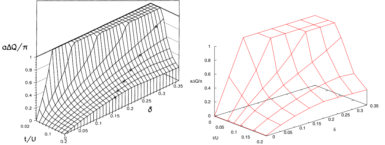
Fig. 3. A benchmark of \Theta\Phi ISS phase diagram against the results of Ref. [6]: (left panel) Ref. [6], (right panel) \Theta\Phi calculations. The axes represent inverse interaction t/U , doping \delta and pitch vector offset from (\pi, \pi) normalized to \pi .
